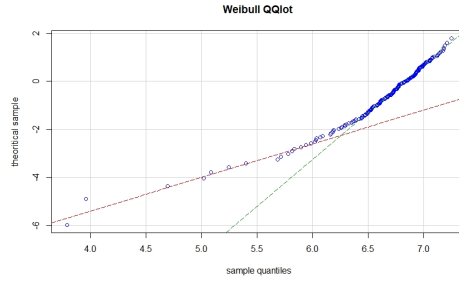
Figure 1: Weibull QQ-plot for competing risks data: the QQ-plot is convex and for small t , R_{WCR} \simeq R(t|\beta_1; \eta_1) and for large t , R_{WCR} \simeq R(t|\beta_2; \eta_2) . Thus, the left tangent (right resp.) allows to estimate (\beta_1; \eta_1) ( (\beta_2; \eta_2) resp.) cf. [3]
