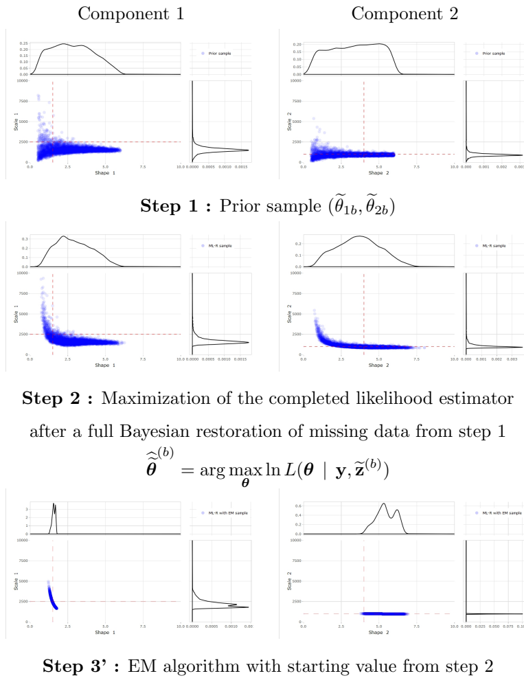
Figure 5: BR-LM with EM algorithm
