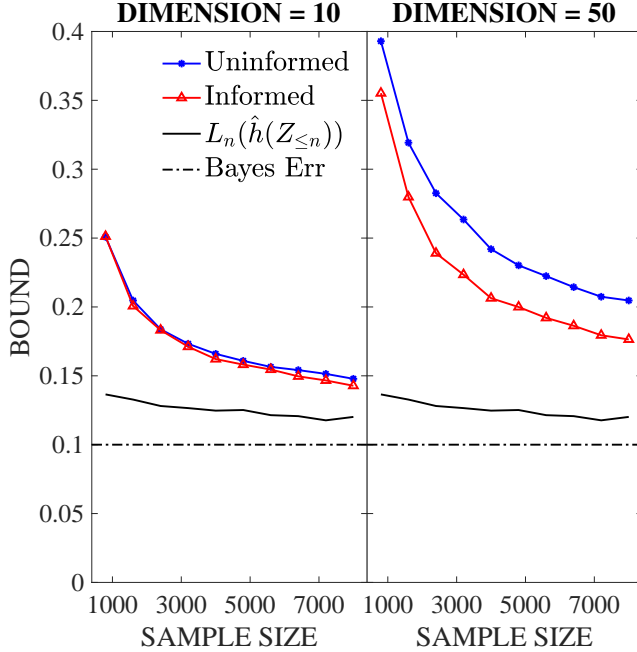
Figure 3: Results for the synthetic data: (Blue curve) Uninformed Maurer’s bound (2); (Red curve) Informed Maurer’s bound (10).
