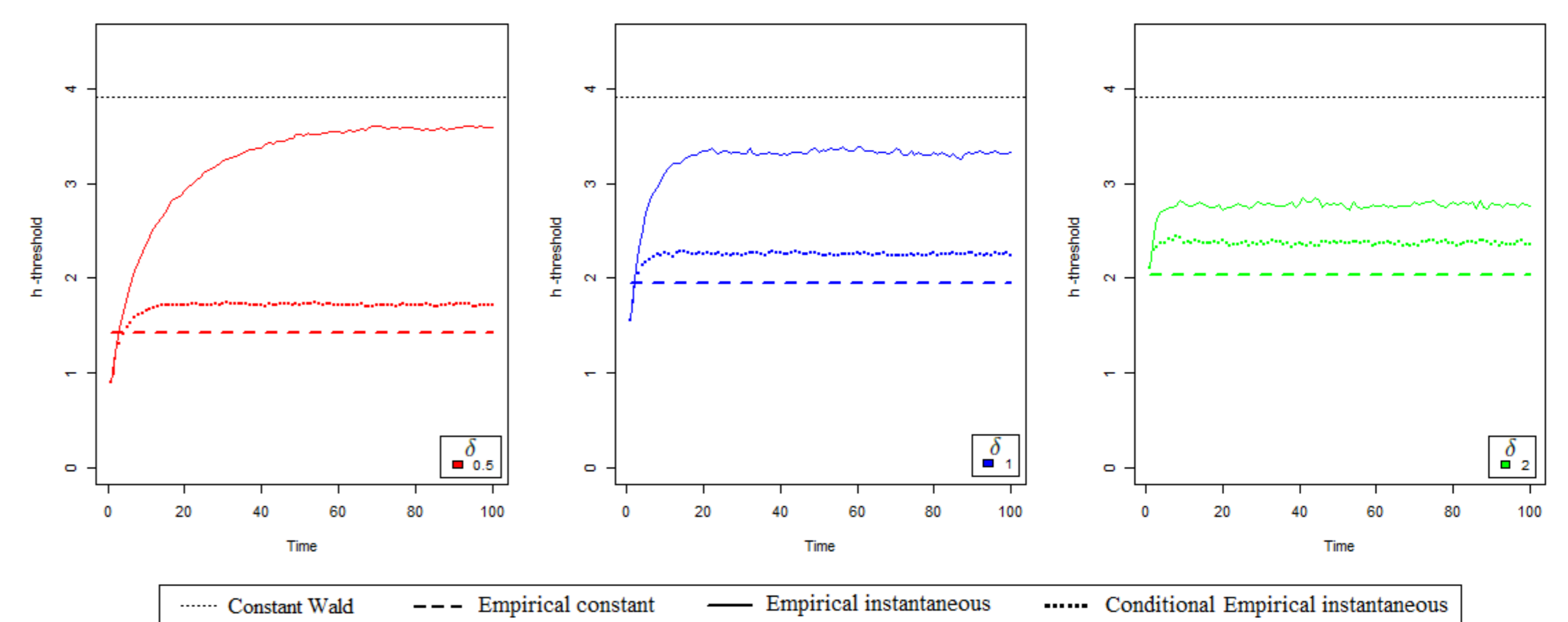
Figure 3: Comparison of the different empirical thresholds and that of Wald, built for \alpha = 0.02 and according to different detection objectives \delta \in \{0.5, 1, 2\} , q = 1 , \sigma_0 = 1 .
