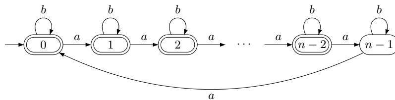
Fig. 4. Witness language T of Definition 1.
