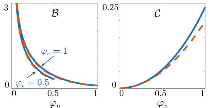
FIG. 3: Interface parameters (\mathcal{B}, \mathcal{C}) ; in plain line, deduced from the numerical resolution of the elementary problems (see Appendix A) and in dotted lines given by the closed forms (4).
