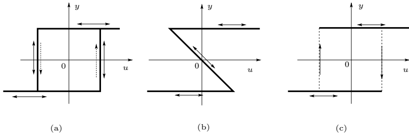
Fig. 2.3: Hysteresis operators.
