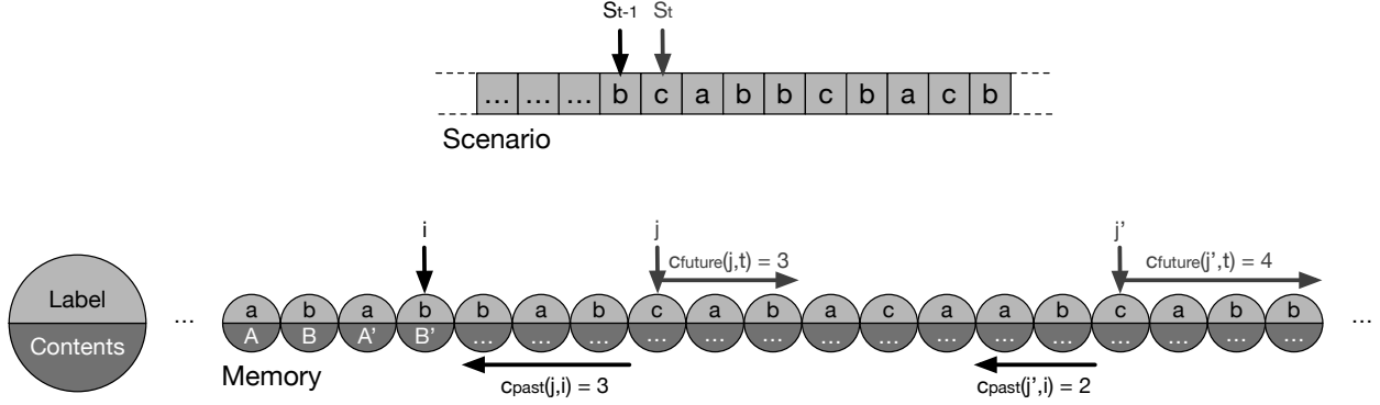
Figure 5. Creation of the set of states in the memory sharing a common future with the current position in the scenario t and a common past with the current event in the memory i_{t-1} for the anticipation step, following Nika et al. (2017a).
