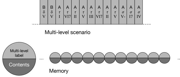
Figure 6. Example of a multi-level scenario and a multi-level memory.
