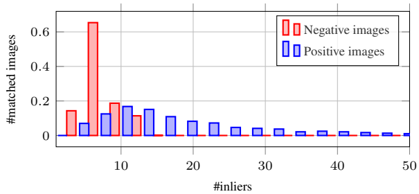
Figure 6. Distribution of number of inliers for positive and negative database images over all queries of \mathcal{ROxf} , using VGG-MAC.
