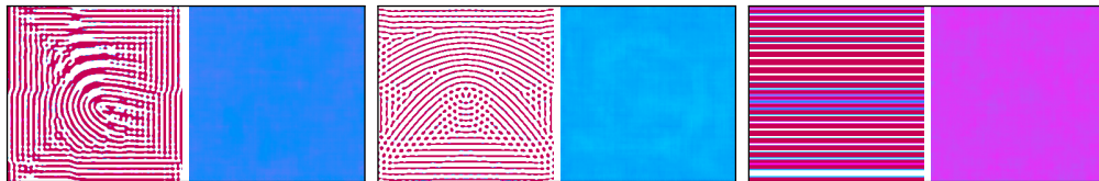
Figure 22: Examples of “textured” patterns that the VAE networks is unable to reconstruct. While a human eye can differentiate the input patterns (spatial frequency, orientation, etc.) the VAE reconstructs all images identically.
