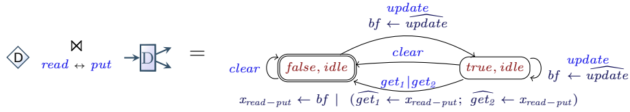
Fig. 3: Example of composition between two Hub Automata, where a DataEvent automaton is composed with a Duplicator automaton by synchronising on actions read and put (left), resulting in the composed automaton on the right.
