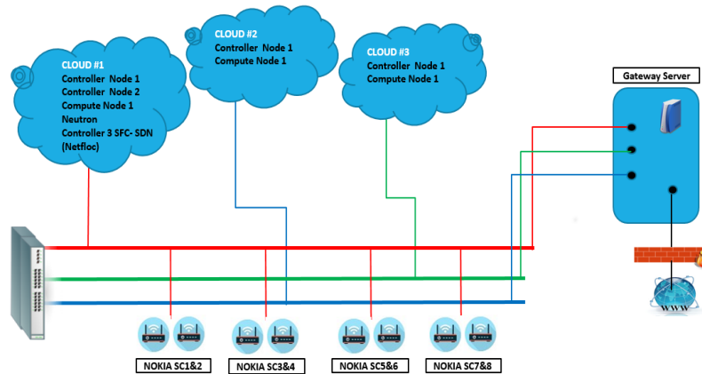
Fig. 3. Topology of the testbed in OTE premises
