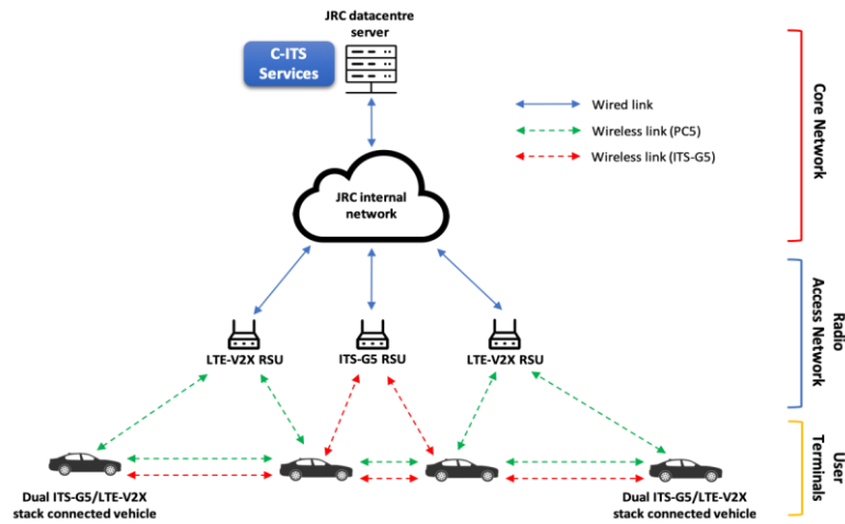
Fig. 6. The ITS-G5/LTE-V2X Testbed at JRC Ispra, in Italy.
