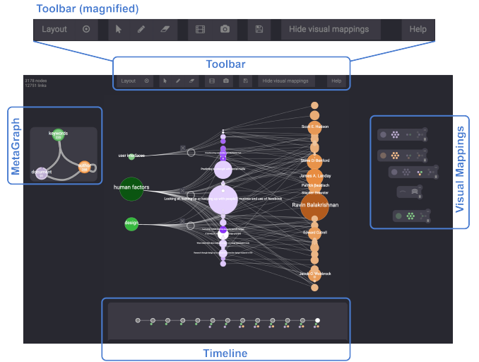
Fig. 2. Graphies: main user interface components. The MetaGraph, Visual Mappings and Timeline are organized on independent layers.
