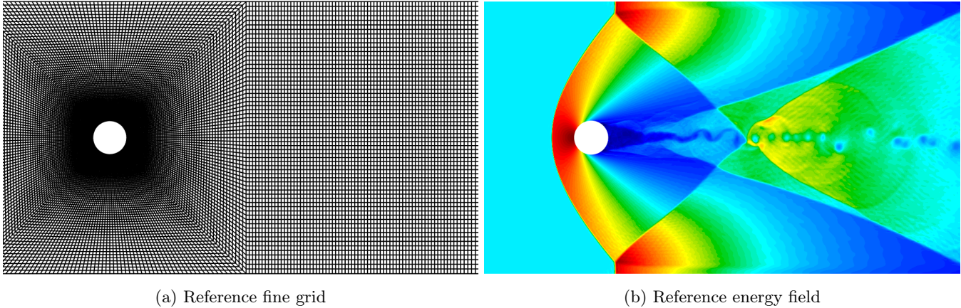
Figure 17: Reference results for the supersonic test-case.
