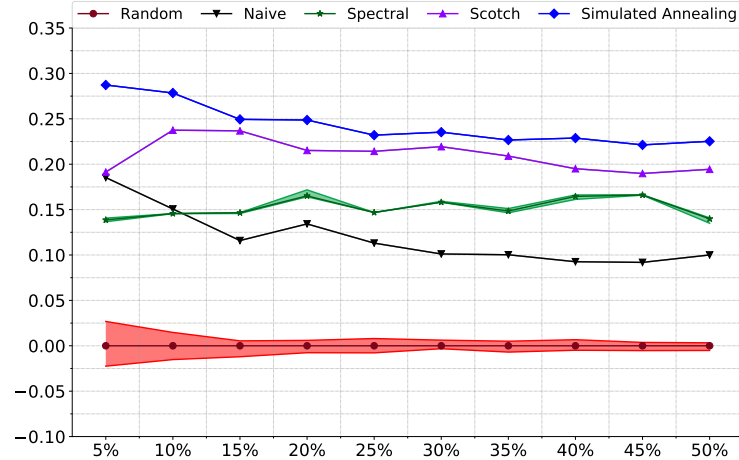
(a) Exploration with 200 neurons per node and fine-grain target graph
