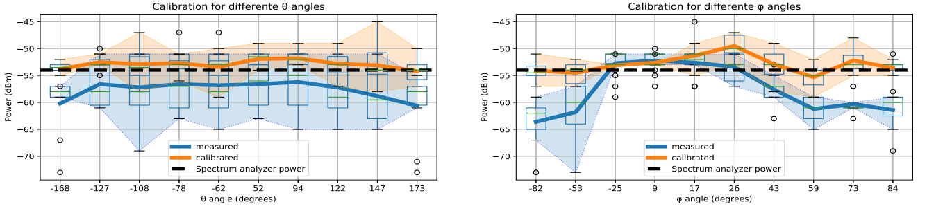
Figure 10: Boxplots for calibration results of the 100 random orientations along \theta and \phi . The calibrated signal (orange) is closer to the reference power (black dashed line), and less variable compared to the raw measured signal (in blue). The colored area represents the variability range of measurements. The RMSE for the calibrated values is 2.4 dBm compared to 6.4 dBm error for the raw measurements.
