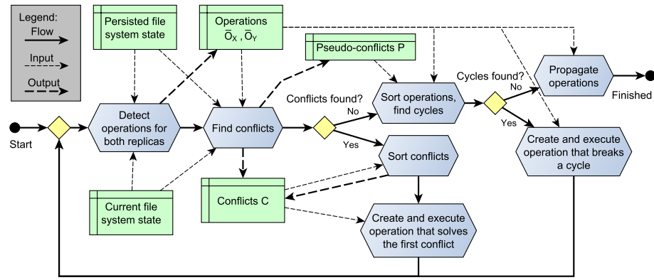
Fig. 1. Synchronization algorithm
