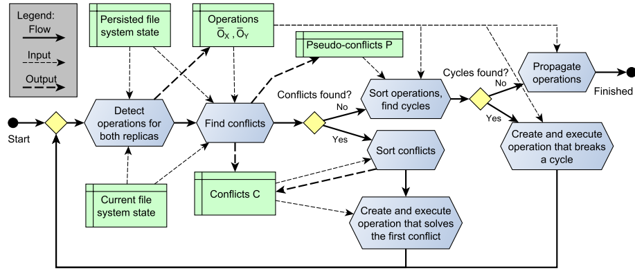
Fig. 1. Synchronization algorithm
