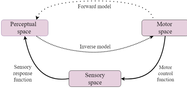
Fig. 1. Sensorimotor model with a perception-action loop. The motor control function generates a sensory representation (a sound in the more complete models) given the motor command parameters. This kind of sensorimotor model includes an inverse model, and potentially a forward model. One of the advantages of a forward model is that it can bias the perceptual representation in order to facilitate the inverse model learning towards perceptuo-motor representations [6].
