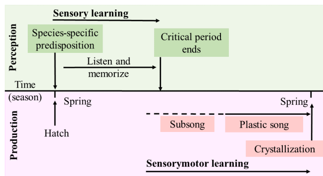
Fig. 4. Imitative learning phases in birds. Three main phases characterise imitative learning in songbirds: the sensory learning phase, the sensorimotor learning phase (in which subsong appears), and crystallization of the sound. Image adapted from Doupe and Kuhl [8].
