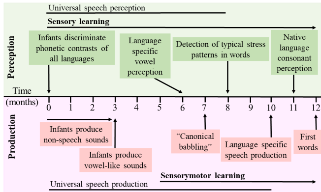
Fig. 3. First year of infant speech-perception and speech-production development. Schema of the first year of infant vocal development. Speech perception development (green background) is characterised by a sensory learning phase for the whole period. Speech production development (pink background) is characterised by some preliminary phases followed by sensorimotor learning, where “canonical babbling” takes place. Image adapted from Kuhl (2004) [4].
