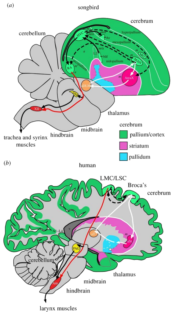
Fig. 5. Brain pathways controlling a) song in songbirds and b) spoken language in humans. The posterior vocal motor pathway (plain black arrows) is also called vocal production pathway, since it involves direct projections to motoneurons. The anterior vocal learning pathway (plain white arrows) is responsible for vocal imitation and plasticity. In addition, there are the connections between the two pathways (dashed black arrows) and specialised direct projection to vocal motor neurons (plain red arrows). Image from Chakraborty and Jarvis (2015) [13].
