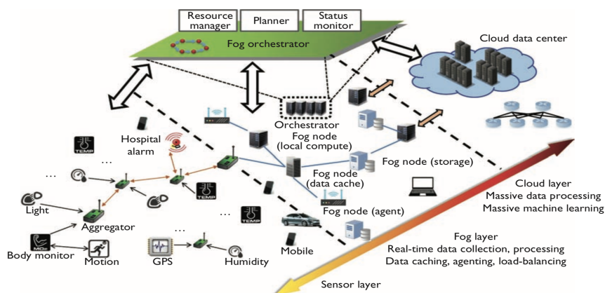
Figure 1: Generic Fog computing architecture [149].
