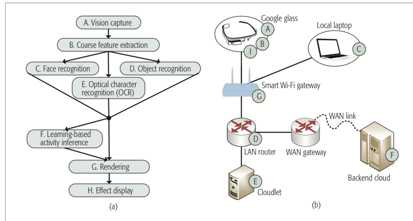
Figure 3: Cognitive assistance application [65], shown in (a), and deployed onto Fog network, shown in (b).
