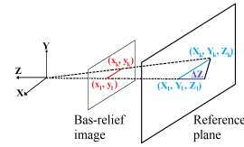
Figure 4: Orthographic projection of a bas-relief.
