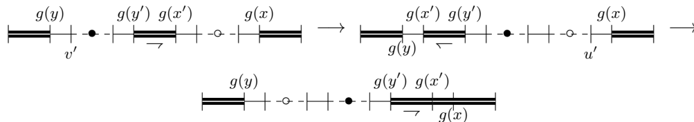
■ Figure 29 Elimination of a jumping pair among two, with two mirror- E -swaps
