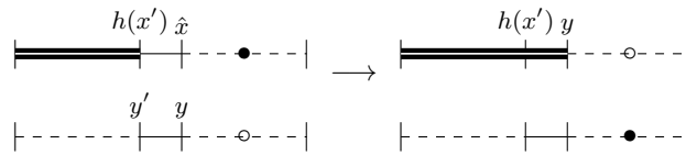
■ Figure 10 y is on a thread disjoint from \text{Im}(h) : we use a crossing- E -swap
