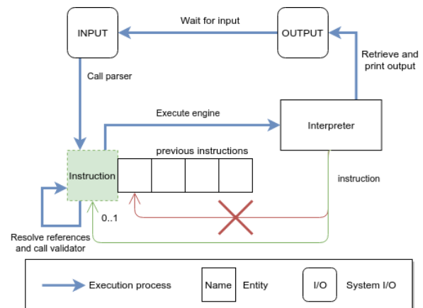
Figure 10. REPL Execution
