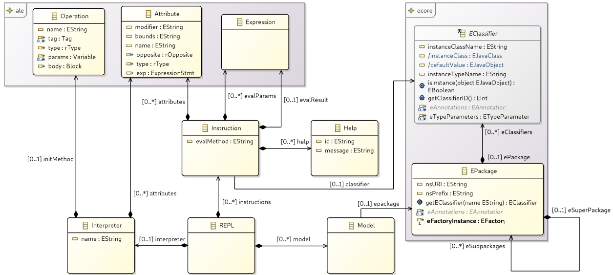
Figure 2. ReplDefinition Metamodel
