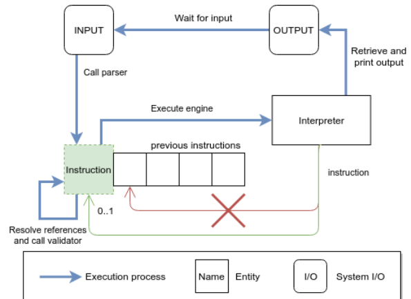
Figure 10. REPL Execution
