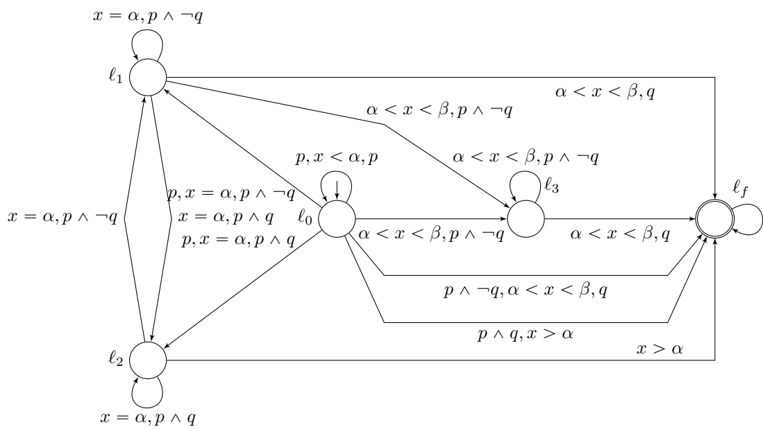
■ Figure 5 Another DTA specification of pU^{\alpha, \beta}q with \alpha > 0 .
