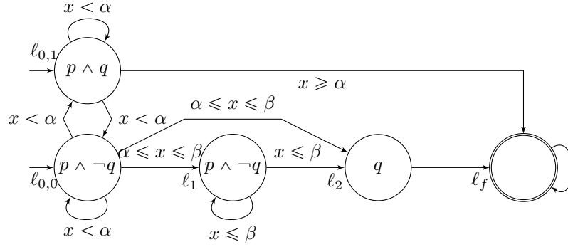
■ Figure 3 Elimination of autonomous transitions with no reset.
