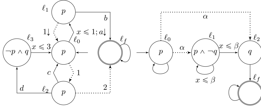
■ Figure 1 Two examples of DTA.
