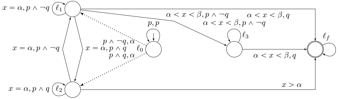
■ Figure 4 A DTA specification of p\mathbf{U}^{\alpha, \beta}q with \alpha > 0 .
