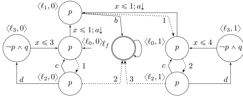
■ Figure 2 Elimination of resetting autonomous transitions.
