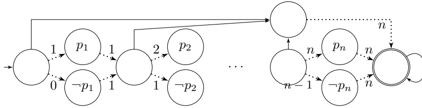
■ Figure 3 Elimination of autonomous transitions with no reset.
