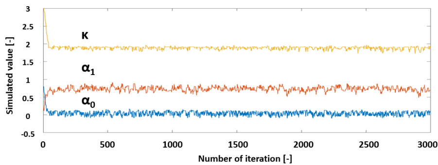
Fig. 5 Trace plots of the parameter as a result of MCMC simulation [11]
