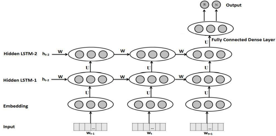
Fig. 1. Proposed LSTM module
