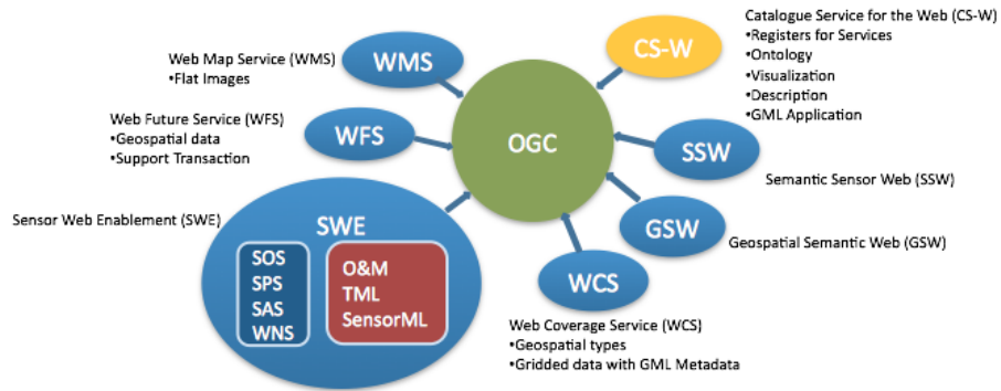
Figure 4: OGC standards schematic view. Definition available at http://www.openeospatial.org/standards/http://www.openeospatial.org/standards/
