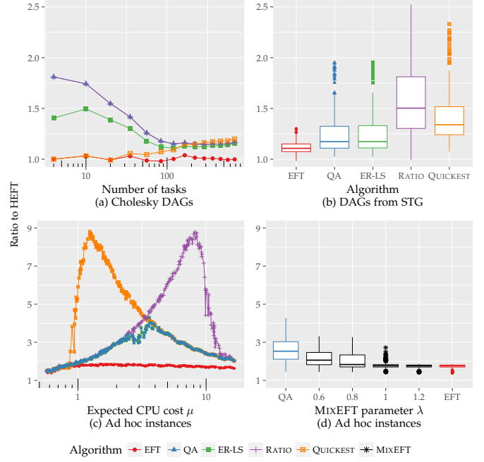
Figure 8. Ratios of the makespan over HEFT for EFT, QA, ER-LS, RATIO, QUICKEST, and MIXEFT with m = 20 CPUs and k = 2 GPUs. Except in Figure (d), MIXEFT is not shown because it performs exactly as EFT. In Figure (d), ER-LS, RATIO, and QUICKEST are discarded.
