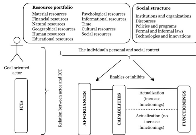
Figure 1. Integrated framework
