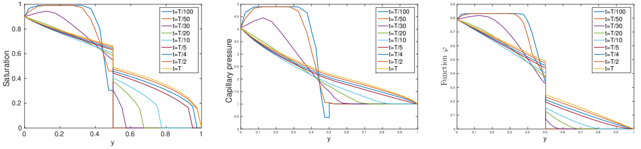
Figure 6.3: Example 1. From left to right: evolution of the saturation, capillary pressure and diffusion function along a line orthogonal to the interface.
