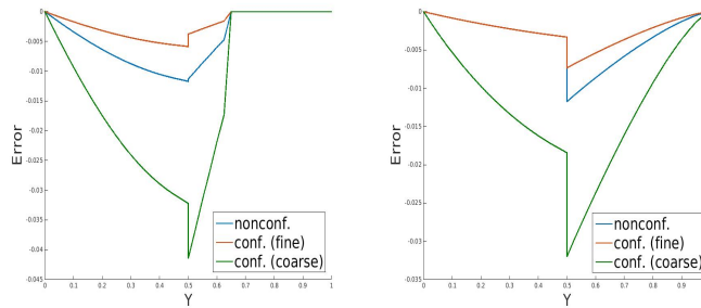
Figure 6.4: Example 1. Error in saturation along a line orthogonal to the interface, nonconforming and conforming (coarse and fine) time-steps. Left T = T_f/20 , right, T = T_f .
