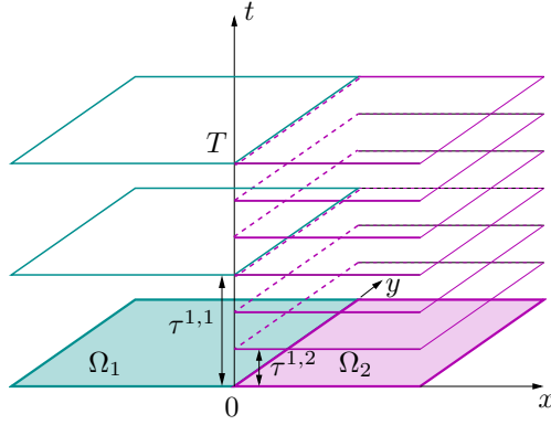
Figure 5.2: Nonconforming time grids between two subdomains \Omega_1 and \Omega_2
