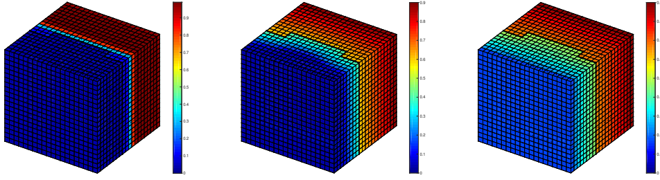
Figure 6.1: Example 1: saturation u(t) , for t = 0.019 , t = 0.3 and t = 3
