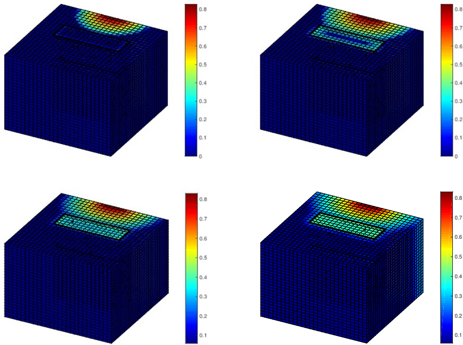
Figure 6.7: Example 2: Saturation u(t) , for t = 100 , t = 200 , t = 350 , t = 480
