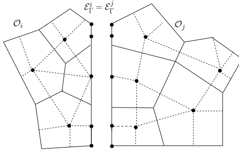
Figure 5.1: Partition of the domain with conforming space grids.
