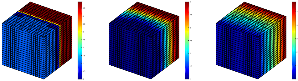
Figure 6.2: Example 1: Capillary pressure \pi(u(t)) , for t = 0.019 , t = 0.3 and t = 3
