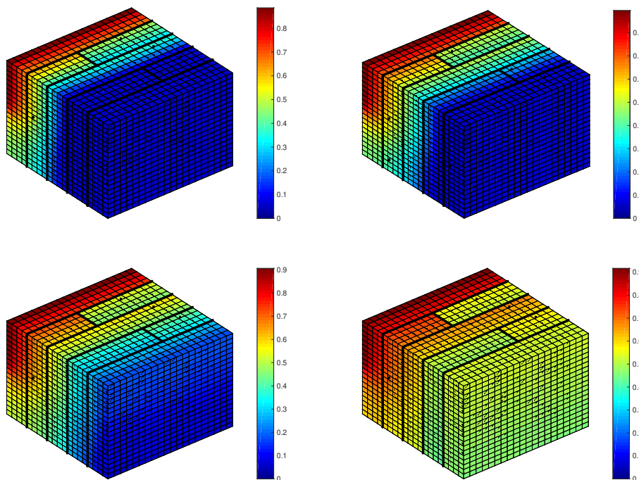
Figure 6.11: Example 3: Saturation u(t) , for t = 500 , t = 1000 , t = 2000 and t = 4000
