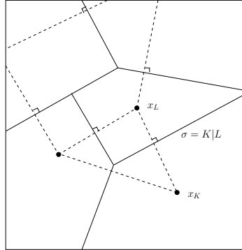
Figure 4.1: Notation for admissible meshes in two space dimensions
