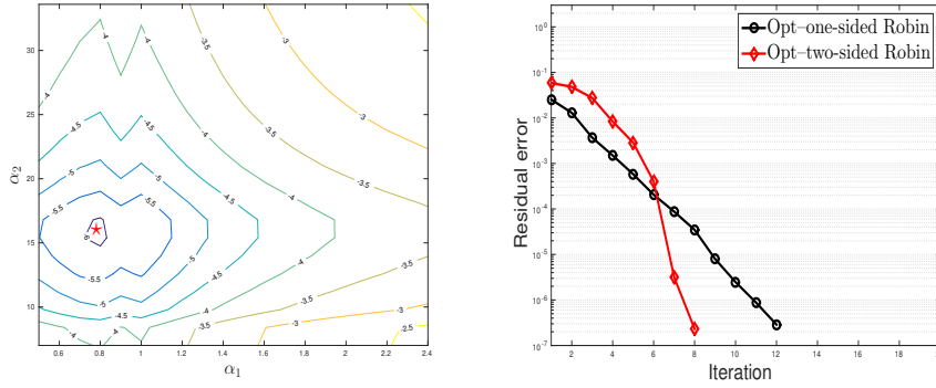
Figure 6.9: Example 2: Left: Level curves for the residual error obtained after 8 iterations for various values of the parameters \alpha_1 and \alpha_2 . The red star shows the optimized parameters. Right: The convergence curves of the optimized Schwarz method with one-sided optimized Robin conditions and two-sided optimized Robin conditions.
