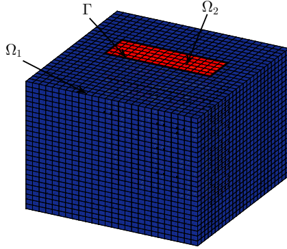
Figure 6.6: Example 2: The geometry and the mesh
