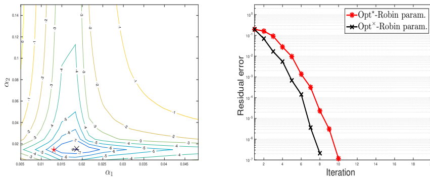
Figure 6.5: Example 1: Left: Level curves for the residual error obtained after 10 iterations for various values of the parameters \alpha_1 and \alpha_2 . The star (in red) marked the parameters obtained with the minimization process of the convergence factor applied to the linearized problem which is close to the best one marked by times symbol (in black). Right: The convergence curves.
