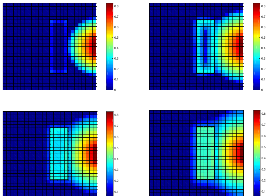
Figure 6.8: Example 2: Saturation u(t) on a slice at the middle of the domain \Omega in the z -direction, for t = 100 , t = 200 , t = 350 , t = 480
