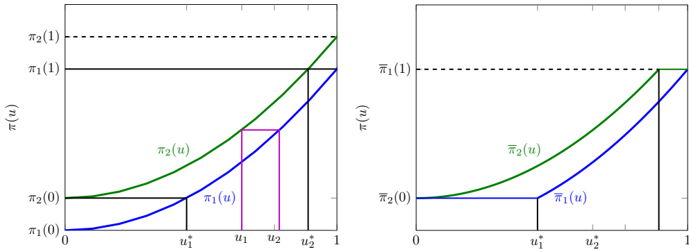
Figure 2.1: Capillarity pressure curves (left) and truncated capillarity pressures curves (right)
