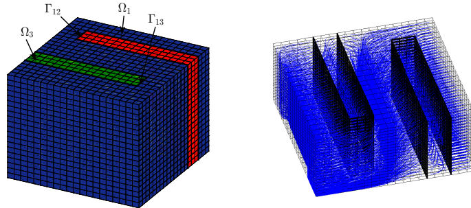
Figure 6.10: Example 3: Left: The geometry and the mesh. Right: Velocity streamlines.
