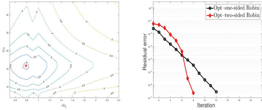
FIG. 6.9. Example 2: Left: Level curves for the residual error obtained after 8 iterations for various values of the parameters \alpha_1 and \alpha_2 . The red star shows the optimized parameters. Right: The convergence curves of the optimized Schwarz method with one-sided optimized Robin conditions and two-sided optimized Robin conditions.
