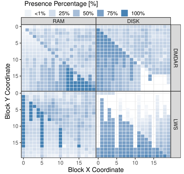
Fig. 14: Heatmaps showing block presence throughout the run.
