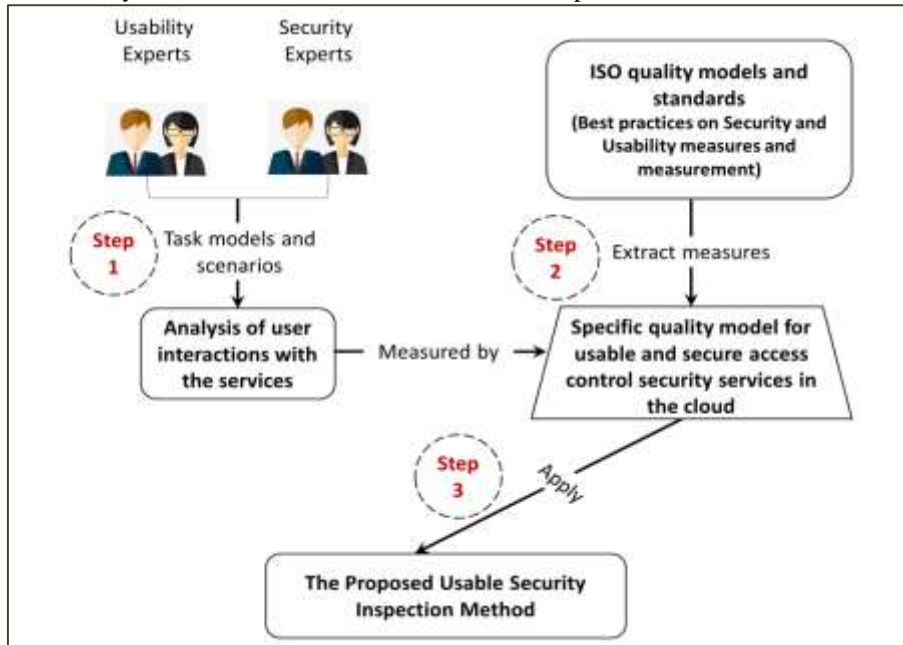
Fig. 1. The proposed usable security measurement methodology
