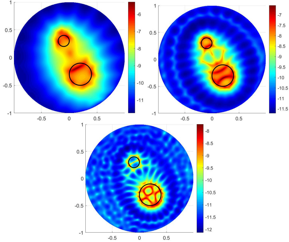
Figure 2: Dirichlet obstacle, exact data and various wave numbers k . Top left: k = 10 . Top right: k = 20 . Bottom: k = 30
