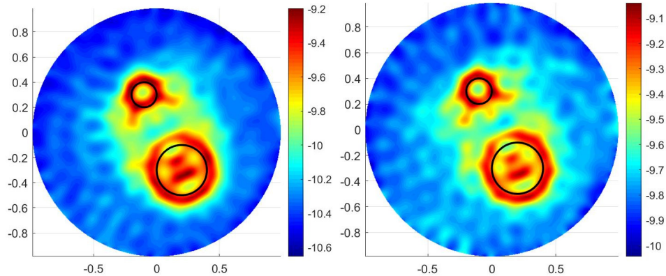
Figure 7: Dirichlet obstacle with less data, k = 20 . Left: noise of amplitude 5%. Right: noise of amplitude 10%.
