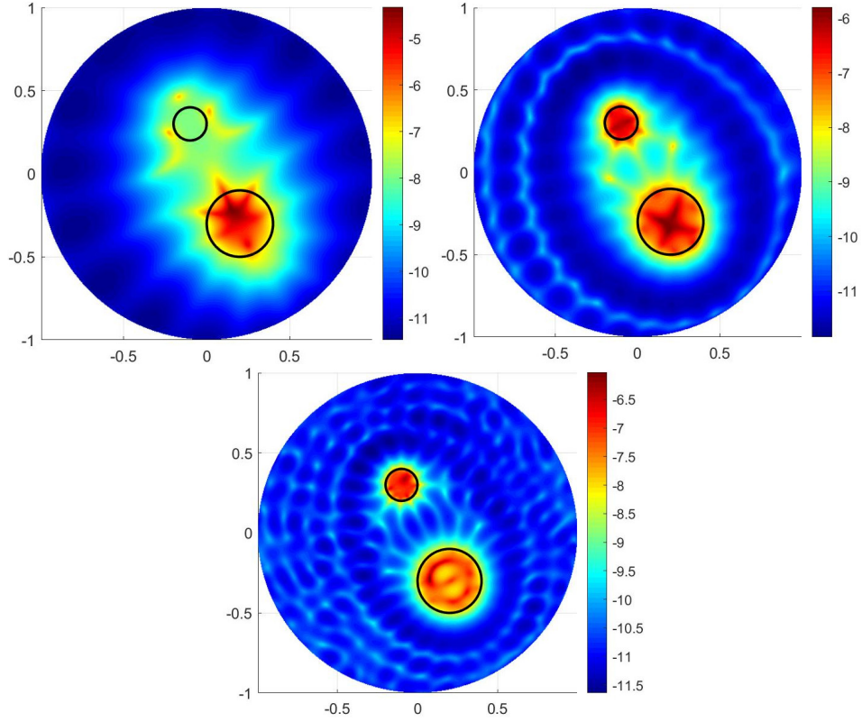
Figure 3: Neumann obstacle, exact data and various wave numbers k . Top left: k = 10 . Top right: k = 20 . Bottom: k = 30 .
