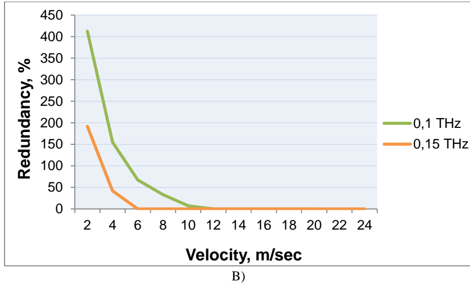
Fig. 4. Dependence of packet losses (A) and redundancy (B) on the UAV's velocity at the transmission frequencies of 0,1 THz and 0,15 THz ( D = 0,5 m)
