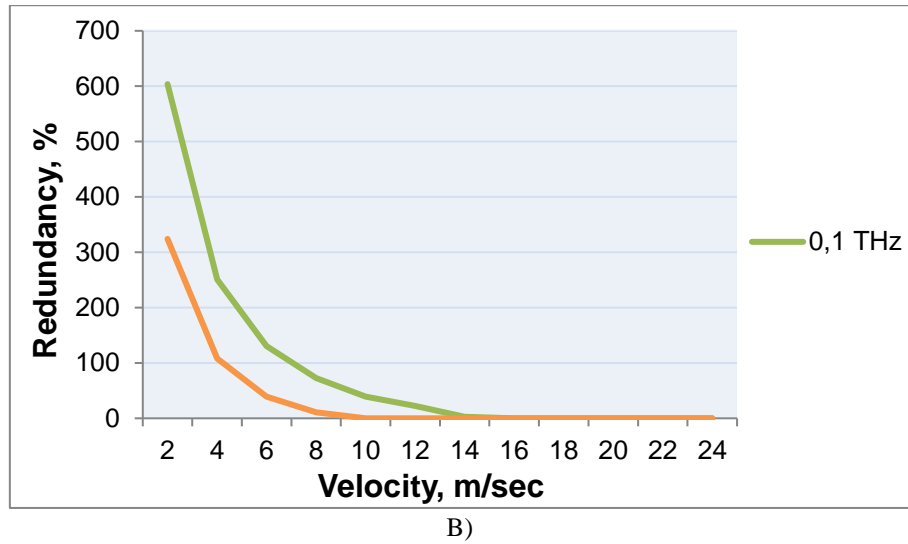
Fig. 3. Dependence of packet losses (A) and redundancy (B) on the UAV's velocity at the transmission frequencies of 0,1 THz and 0,15 THz ( D = 0,4 m)
