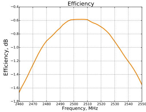
Fig. 14. Radiation efficiency
