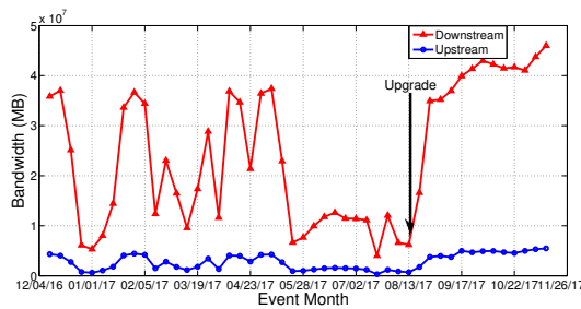
Fig. 2. Network Traffic
