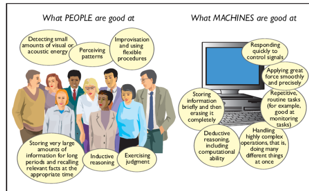
Fig. 2. Best player between human and computer from Carver and Tuross [25]
