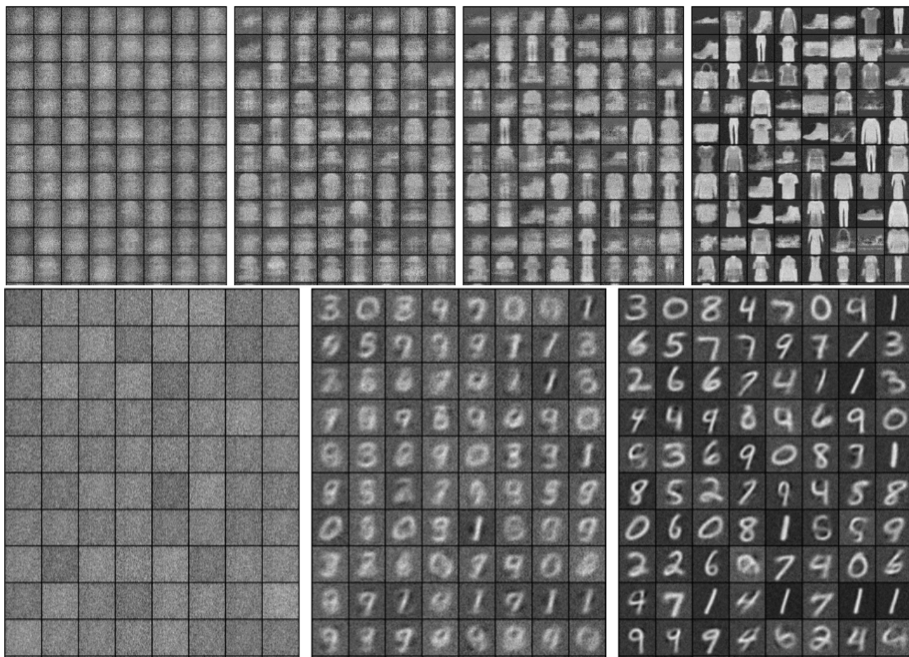
Figure S1. The evolution of SWF through 15000 iterations, when the original high-dimensional data is kept instead of working on reduced bottleneck features as done in the main document. Showing results on the MNIST and FashionMNIST datasets. For a visual comparison for FashionMNIST, we refer the reader to (Samangouei et al., 2018).
