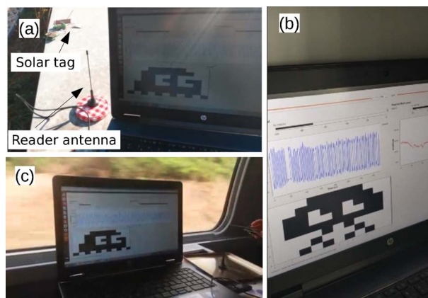
Figure 1. Photos of (a) Sun-powered TV backscatter (b) 4G backscatter (c) TV backscatter on board of a Paris-to-Lyon high speed train,
