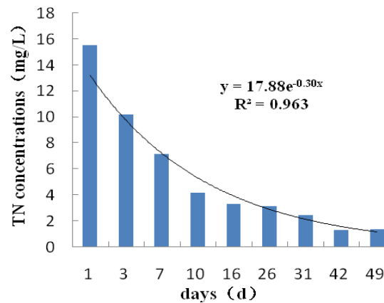
Fig. 7. TN reduction law of combination 5 (exponential fitting)
