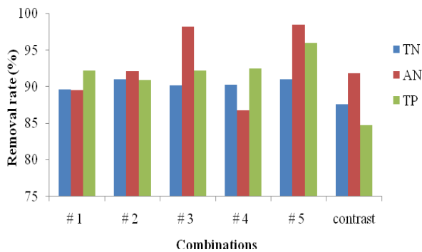
Fig. 5. Nitrogen and phosphorus removal rate
