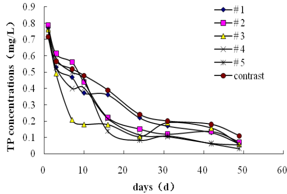
Fig. 4. TP concentration changes in water
