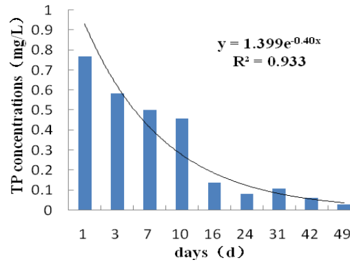
Fig. 9. TP reduction law of combination 5 (exponential fitting)
