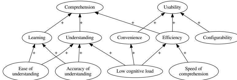
Fig. 4: Goal decompositions that are derived from the top-goals Comprehension and Usability of a visual modeling language
