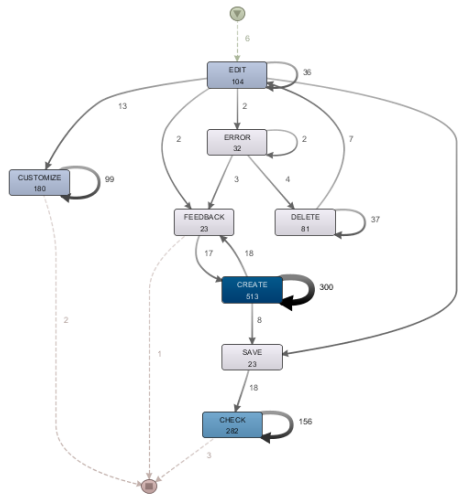
Fig. 9: Process model created in Disco for HW2, low-scoring students, 2017
