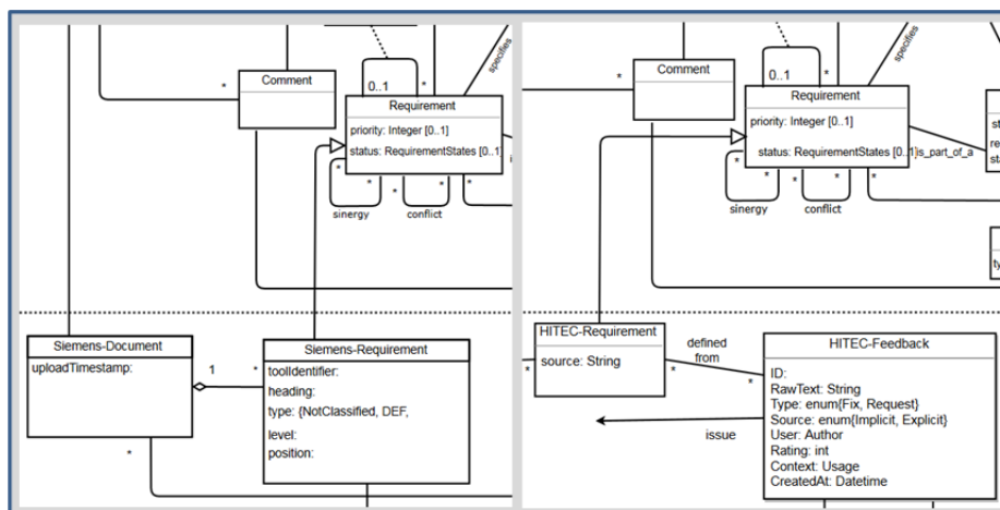
Fig. 6. Mappings with the OpenReq RE domain ontology: (a) mapping SIEMENS requirements; (b) Mapping HITEC user feedback.
