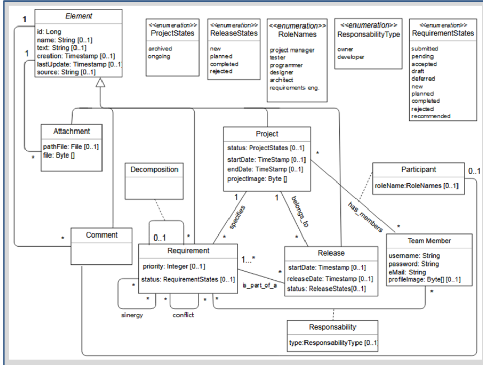
Fig. 5. The OpenReq reference model for requirements engineering.
