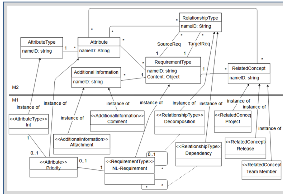
Fig. 7. The OpenReq metamodel for requirements.
