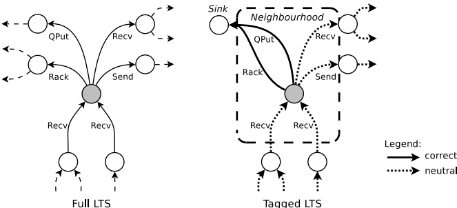
Fig. 5: Example of neighbourhood with correct transitions.
