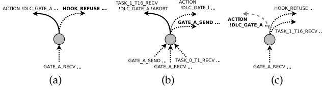
Fig. 17: Multiway rendezvous protocol: three of the neighbourhoods detected in the abstracted counterexample.
