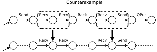
Fig. 9: Example of counterexample abstraction.
