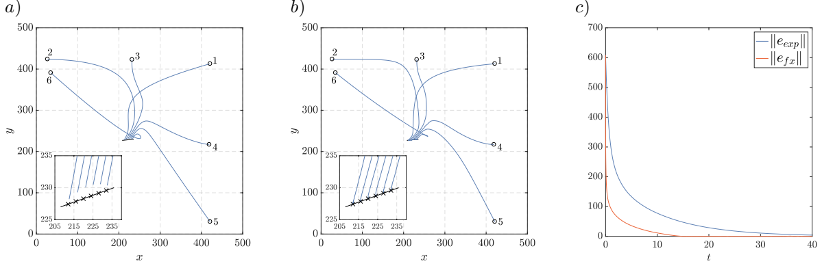
Figure 4: Comparison of systems (17) and (19) with initial conditions x(0) = 208, 241 + d, 207 - d, 232, 239 + d, 241 + d, 215 - d, 236, y = [227, 233 + d, 244 + d, 243 + d, 217, 210 - d, 211 + d, 230] , d = 180 and parameters c_1 = c_2 = 1, \mu = 1.1 for the allocation algorithm (18). a) and b) shows the trajectories (x_i(t), y_i(t)) of systems (17) and (19), respectively. c) depicts a plot of the norm of the distance between the initial points and the target points of each system, denoted \|e_{exp}\| and \|e_{fx}\| , respectively.
