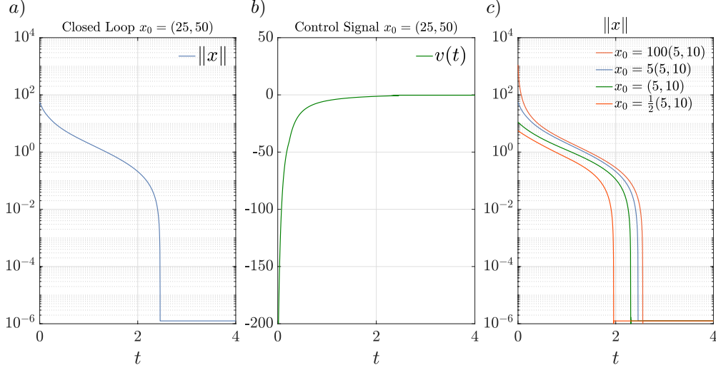
Figure 5: State norm \|x\| in semi-logarithmic scale (a) and the control signal v(t) (b) of the system (30) in closed loop with x_0 = (25, 50) , \nu = \frac{1}{2} and \mu = \frac{1}{5} . The norm of the state in closed loop for four different initial conditions is depicted in c.
