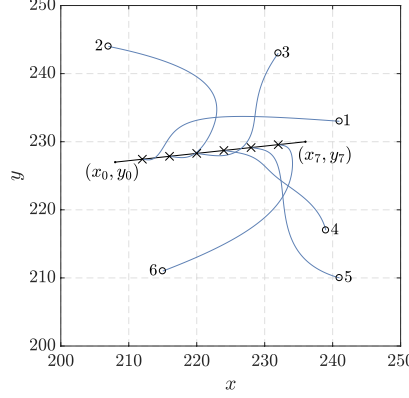
Figure 3: Position trajectories (x_i(t), y_i(t)) of the multi-agent system (17) with n = 6 , initial positions x(0) = [241, 207, 232, 239, 241, 215] , y(0) = [233, 244, 243, 217, 210, 211] and a target line segment given by the points (x_0, y_0) = (208, 227) and (x_7, y_7) = (236, 230) . The symbol \circ denotes the initial position of each agent and \times denotes its target position along the line segment depicted in bold black. The number beside each initial point corresponds to the agent's index i .
