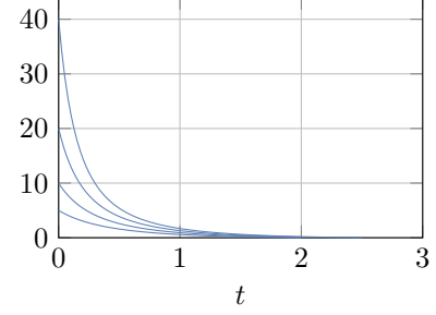
Figure 1: Solutions of system (7) for four different initial conditions.
