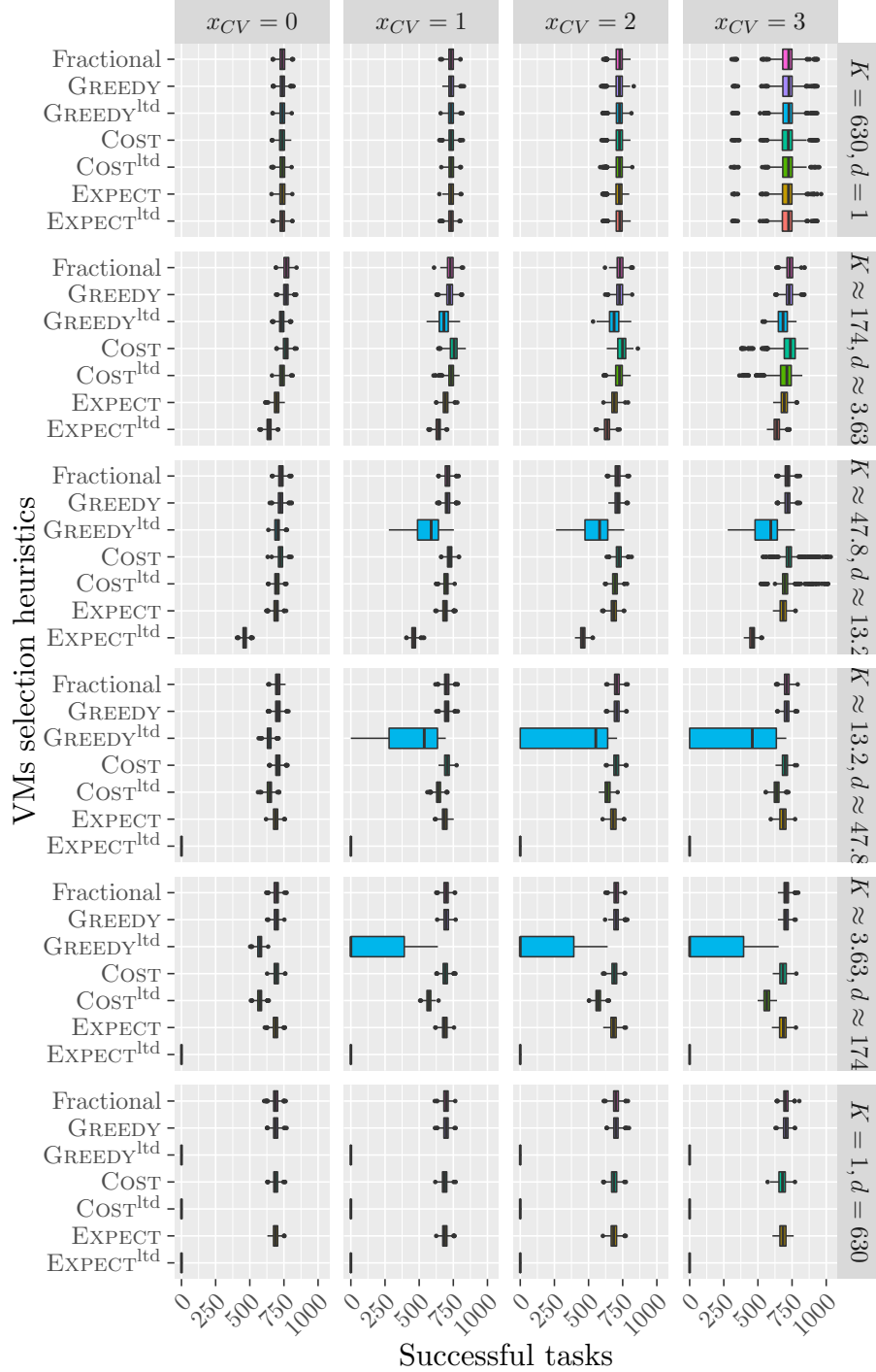
Figure 22: Number of successfully executed tasks of different methods to choose VMs when interrupting tasks with heuristic OPTRATIO. Platforms are generated with m_j = 10 , M = 60 , c_j = s_j , b = 630 . The values for d and K follows a geometric progression between 1 and b = 630 . Execution times follow an inverse gamma distribution.
