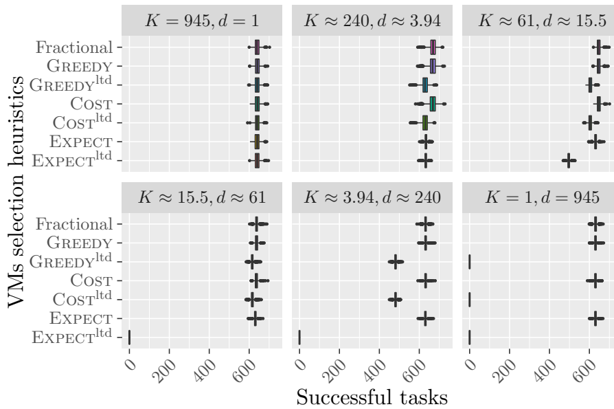
Figure 17: Number of successfully executed tasks of different methods to choose VMs when interrupting tasks with heuristic OPTRATIO. Platforms are generated with m_j = 10 , M = 60 , c_j = 1.5s_j and b = 945 . The values for d and K follows a geometric progression between 1 and b = 945 . Execution times follow an uniform distribution.
