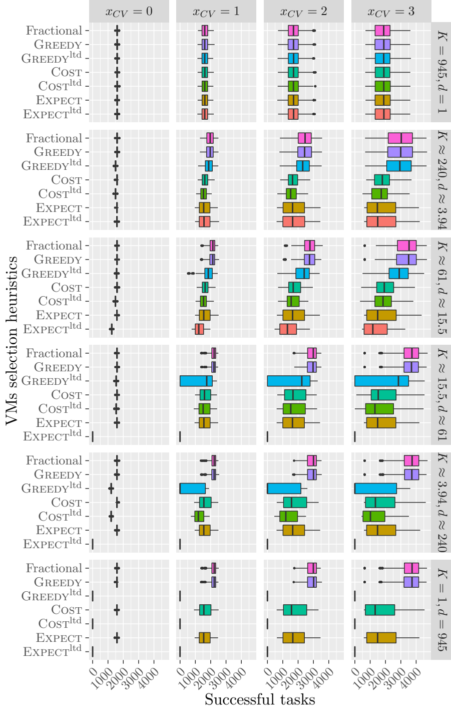
Figure 14: Number of successfully executed tasks of different methods to choose VMs when interrupting tasks with heuristic OPTRATIO. Platforms are generated with m_j = 10 , M = 60 , c_j = 1.5s_j and b = 945 . The values for d and K follows a geometric progression between 1 and b = 945 . Execution times follow a lognormal distribution.
