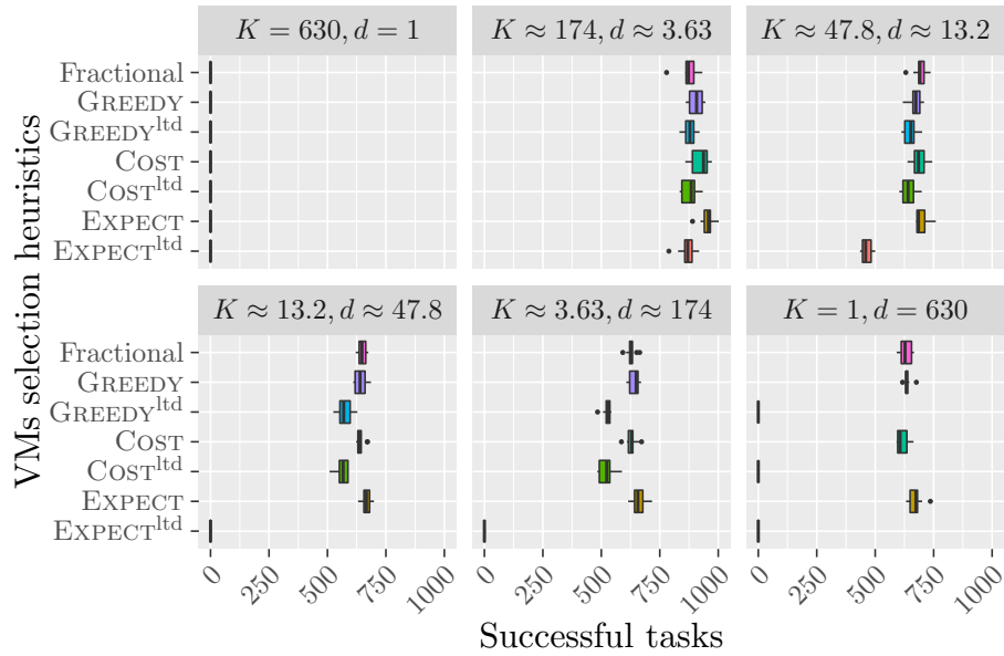
Figure 34: Number of successfully executed tasks of different methods to choose VMs when interrupting tasks with heuristic OPTRATIO. Platforms are generated with m_j = 10 , M = 60 , c_j = s_j , b = 630 . The values for d and K follows a geometric progression between 1 and b = 630 . Execution times follow an exponential distribution.
