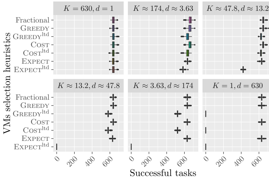
Figure 16: Number of successfully executed tasks of different methods to choose VMs when interrupting tasks with heuristic OPTRATIO. Platforms are generated with m_j = 10 , M = 60 , c_j = s_j , b = 630 . The values for d and K follows a geometric progression between 1 and b = 630 . Execution times follow an uniform distribution.
