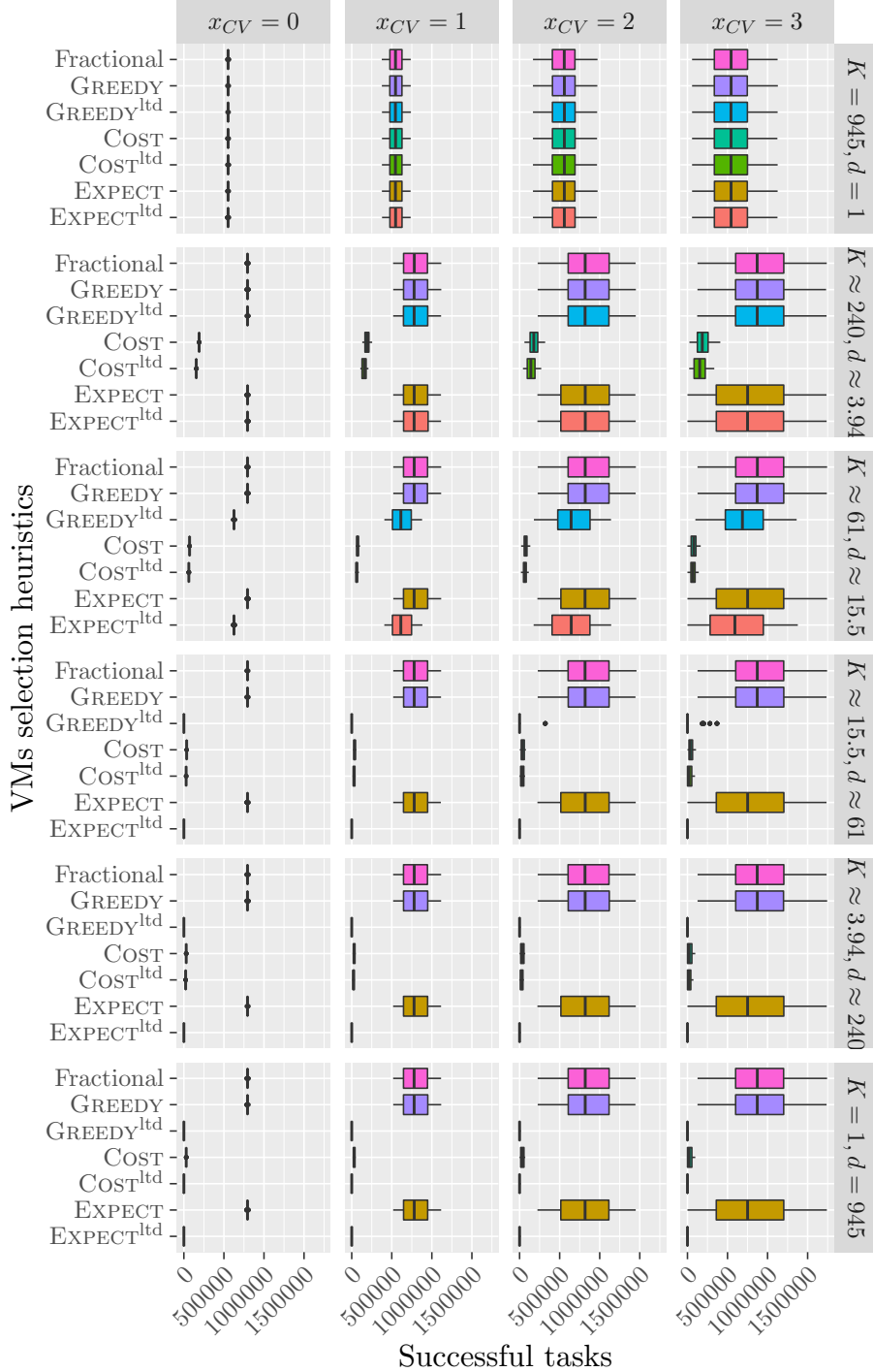
Figure 26: Number of successfully executed tasks of different methods to choose VMs when interrupting tasks with heuristic OPTRATIO. Platforms are generated with m_j = 10 , M = 60 , c_j = 1.5s_j and b = 945 . The values for d and K follows a geometric progression between 1 and b = 945 . Execution times follow a gamma distribution.
