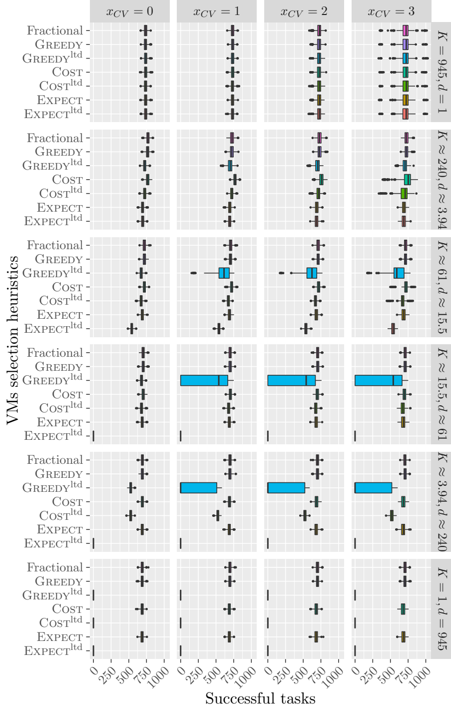
Figure 23: Number of successfully executed tasks of different methods to choose VMs when interrupting tasks with heuristic OPTRATIO. Platforms are generated with m_j = 10 , M = 60 , c_j = 1.5s_j and b = 945 . The values for d and K follows a geometric progression between 1 and b = 945 . Execution times follow an inverse gamma distribution.
