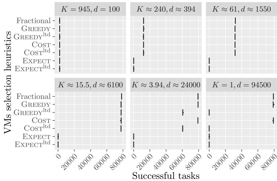
Figure 32: Number of successfully executed tasks of different methods to choose VMs when interrupting tasks with heuristic OPTRATIO. Platforms are generated with m_j = 10 , M = 60 , c_j = 1.5s_j and b = 94500 . The values for d follows a geometric progression between 100 and b = 94500 . Execution times follow a half-normal distribution.
