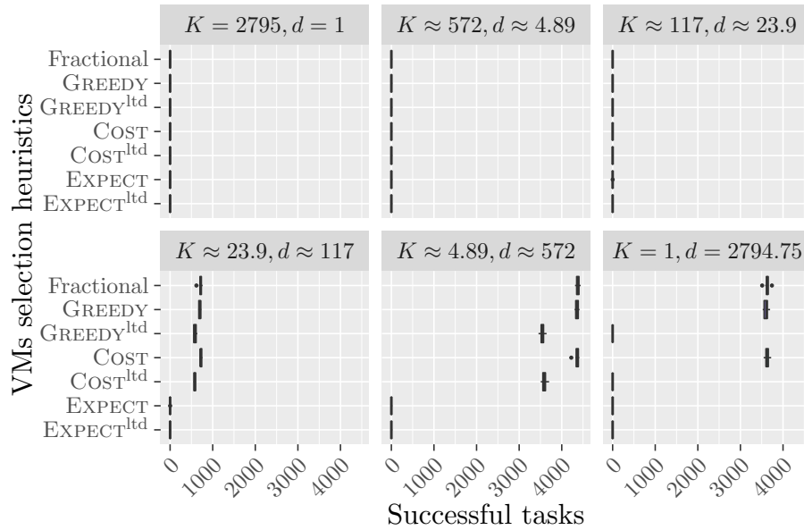
Figure 30: Number of successfully executed tasks of different methods to choose VMs when interrupting tasks with heuristic OPTRATIO. Platforms are generated with m_j = 10 , M = 60 , c_j = s_j^{1.5} and b \approx 2795 . The values for d and K follows a geometric progression between 1 and b \approx 2795 . Execution times follow a half-normal distribution.
