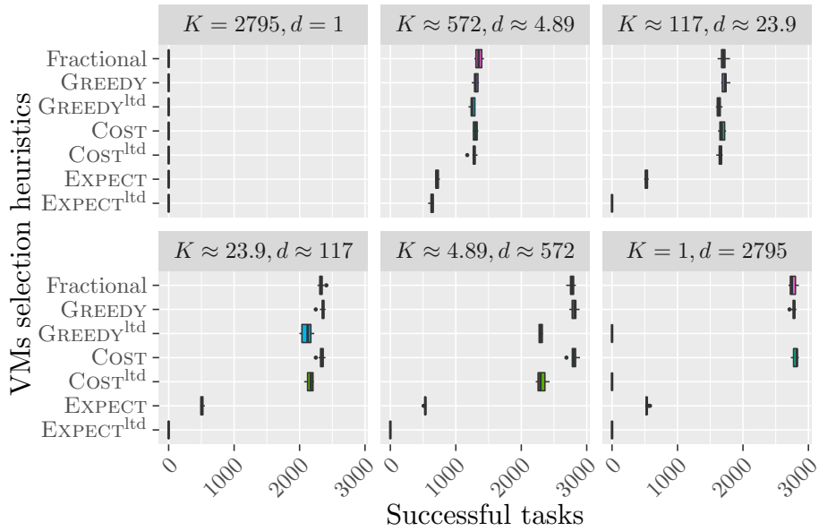
Figure 36: Number of successfully executed tasks of different methods to choose VMs when interrupting tasks with heuristic OPTRATIO. Platforms are generated with m_j = 10 , M = 60 , c_j = s_j^{1.5} and b \approx 2795 . The values for d and K follows a geometric progression between 1 and b \approx 2795 . Execution times follow an exponential distribution.
