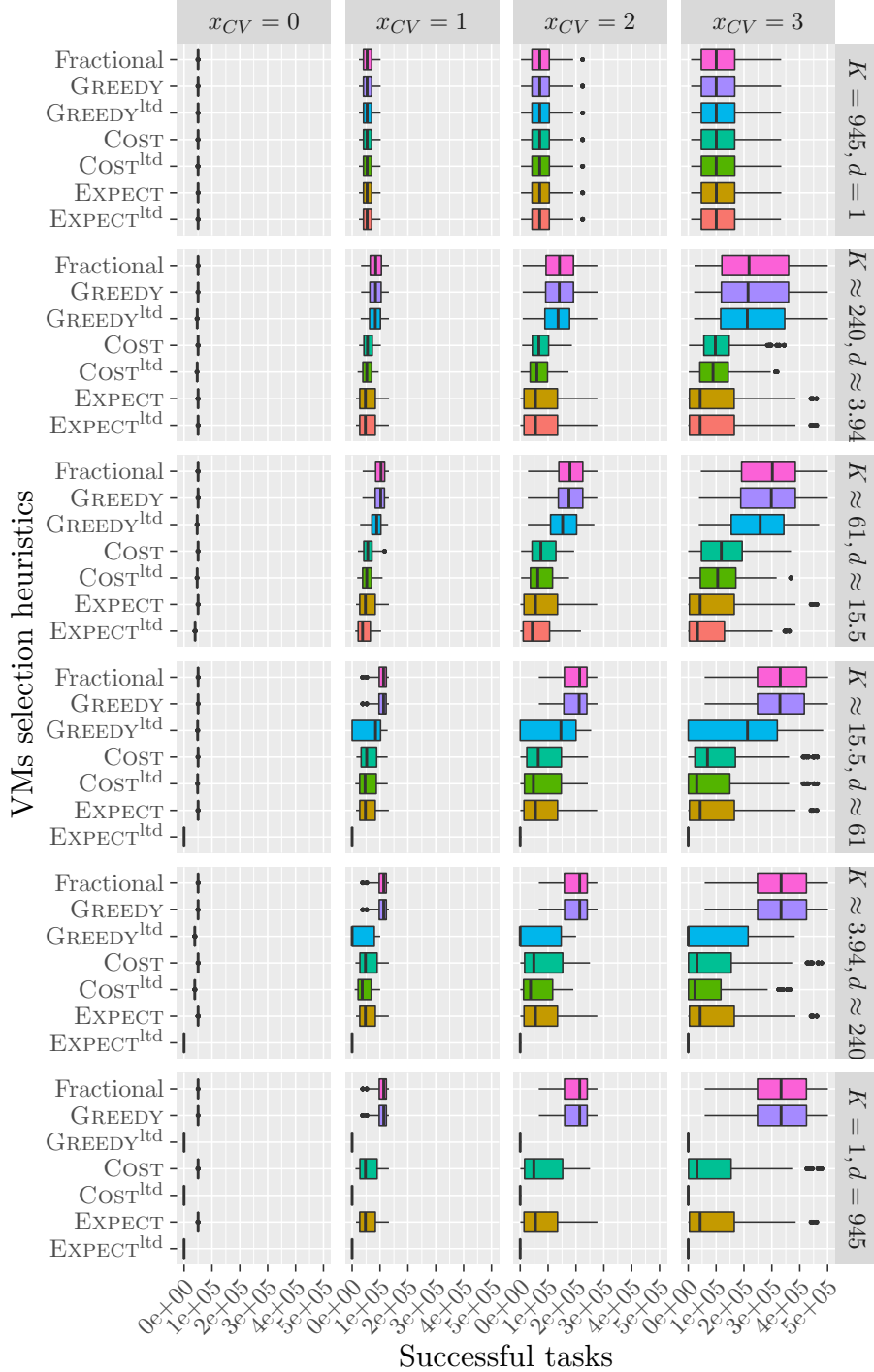
Figure 20: Number of successfully executed tasks of different methods to choose VMs when interrupting tasks with heuristic OPTRATIO. Platforms are generated with m_j = 10 , M = 60 , c_j = 1.5s_j and b = 945 . The values for d and K follows a geometric progression between 1 and b = 945 . Execution times follow a Weibull distribution.
