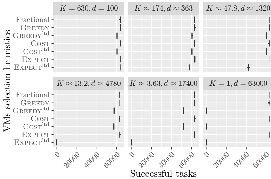
Figure 37: Number of successfully executed tasks of different methods to choose VMs when interrupting tasks with heuristic OPTRATIO. Platforms are generated with m_j = 10 , M = 60 , c_j = s_j , b = 63000 . The values for d follows a geometric progression between 100 and b = 63000 . Execution times follow an exponential distribution.
