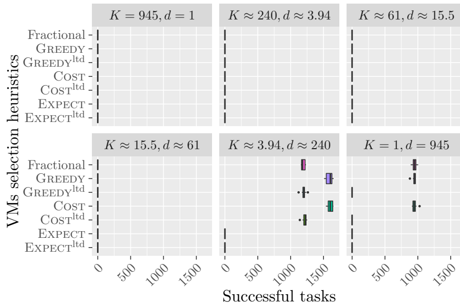
Figure 29: Number of successfully executed tasks of different methods to choose VMs when interrupting tasks with heuristic OPTRATIO. Platforms are generated with m_j = 10 , M = 60 , c_j = 1.5s_j and b = 945 . The values for d and K follows a geometric progression between 1 and b = 945 . Execution times follow a half-normal distribution.
