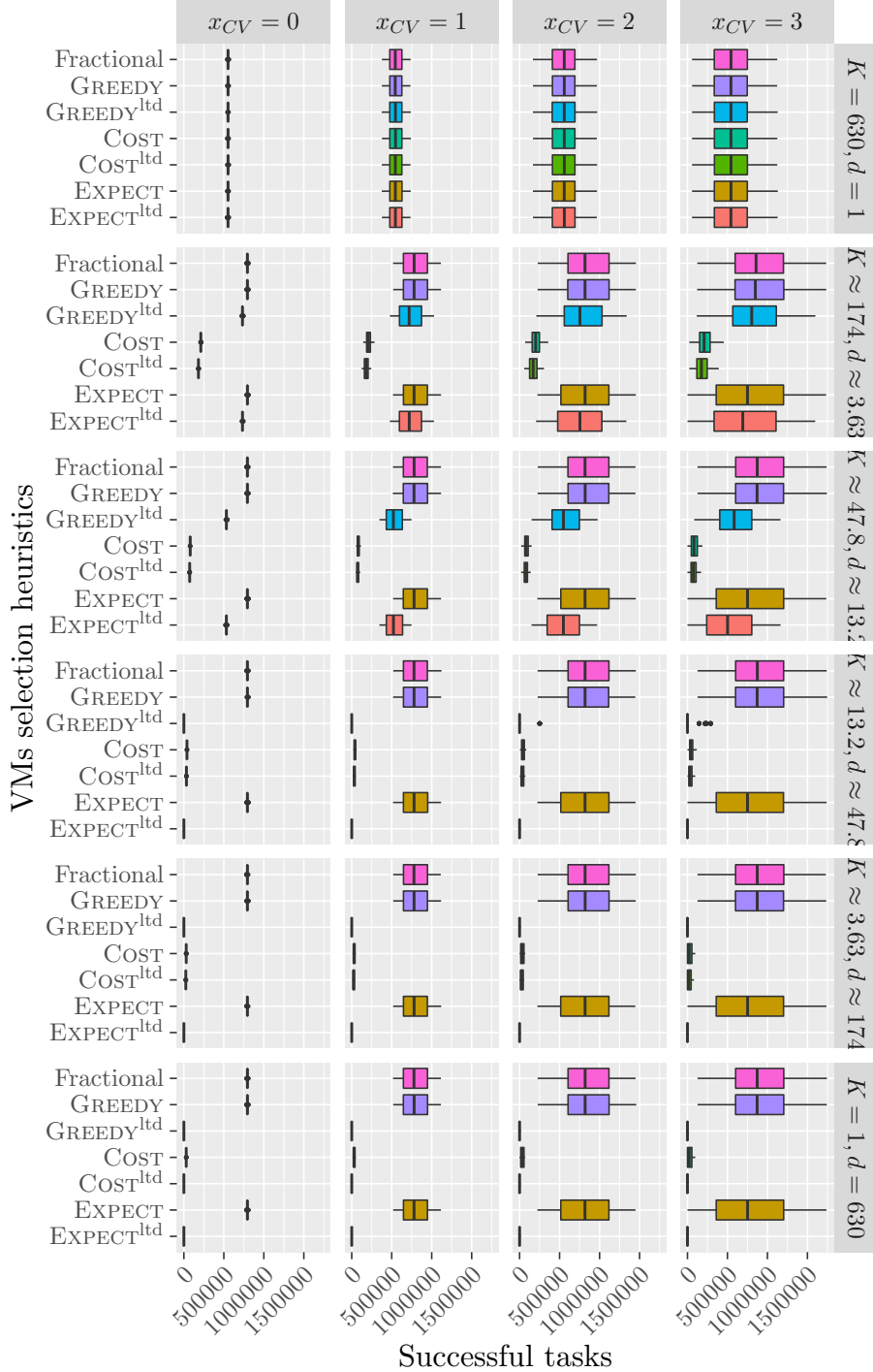
Figure 25: Number of successfully executed tasks of different methods to choose VMs when interrupting tasks with heuristic OPTRATIO. Platforms are generated with m_j = 10 , M = 60 , c_j = s_j , b = 630 . The values for d and K follows a geometric progression between 1 and b = 630 . Execution times follow a gamma distribution.
