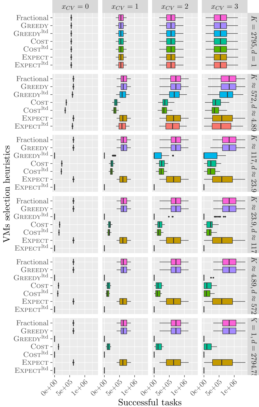
Figure 27: Number of successfully executed tasks of different methods to choose VMs when interrupting tasks with heuristic OPTRATIO. Platforms are generated with m_j = 10 , M = 60 , c_j = s_j^{1.5} and b \approx 2795 . The values for d and K follows a geometric progression between 1 and b \approx 2795 . Execution times follow a gamma distribution.
