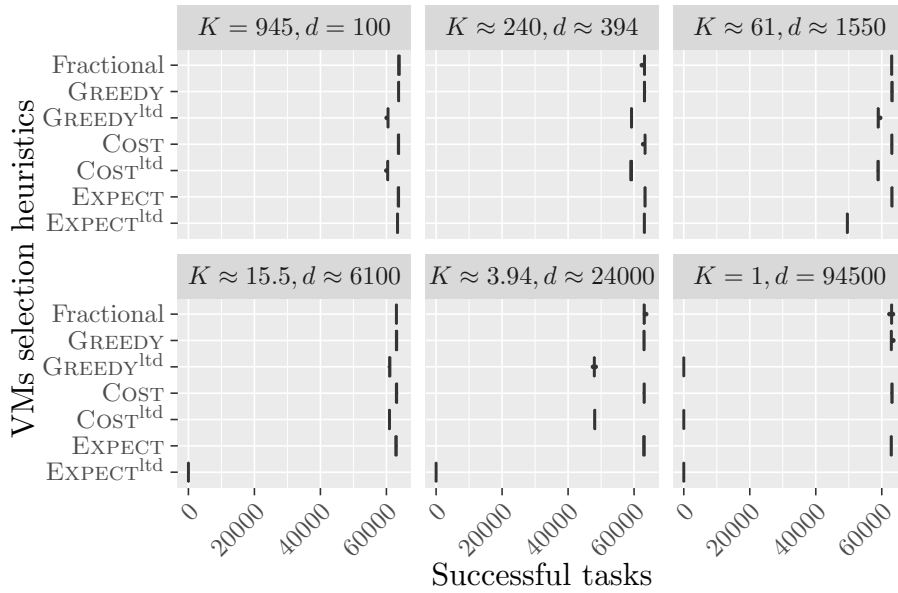
Figure 38: Number of successfully executed tasks of different methods to choose VMs when interrupting tasks with heuristic OPTRATIO. Platforms are generated with m_j = 10 , M = 60 , c_j = 1.5s_j and b = 94500 . The values for d follows a geometric progression between 100 and b = 94500 . Execution times follow an exponential distribution.
