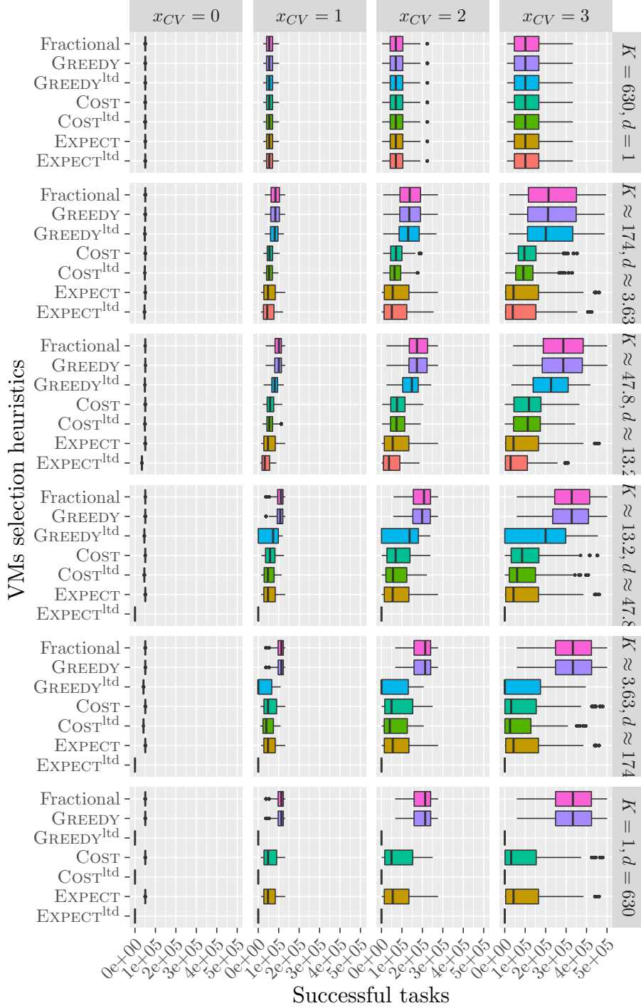
Figure 19: Number of successfully executed tasks of different methods to choose VMs when interrupting tasks with heuristic OPTRATIO. Platforms are generated with m_j = 10 , M = 60 , c_j = s_j , b = 630 . The values for d and K follows a geometric progression between 1 and b = 630 . Execution times follow a Weibull distribution.
