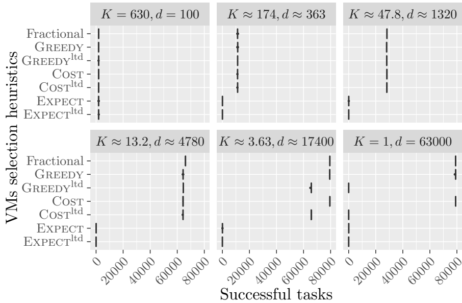
Figure 31: Number of successfully executed tasks of different methods to choose VMs when interrupting tasks with heuristic OPTRATIO. Platforms are generated with m_j = 10 , M = 60 , c_j = s_j , b = 63000 . The values for d follows a geometric progression between 100 and b = 63000 . Execution times follow a half-normal distribution.
