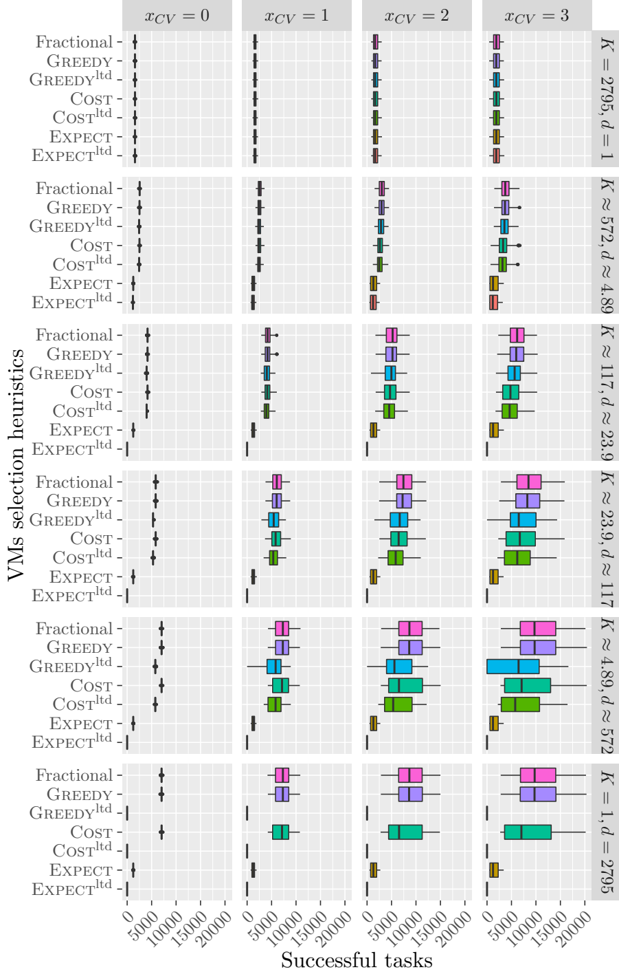
Figure 15: Number of successfully executed tasks of different methods to choose VMs when interrupting tasks with heuristic OPTRATIO. Platforms are generated with m_j = 10 , M = 60 , c_j = s_j^{1.5} and b \approx 2795 . The values for d and K follows a geometric progression between 1 and b \approx 2795 . Execution times follow a lognormal distribution.
