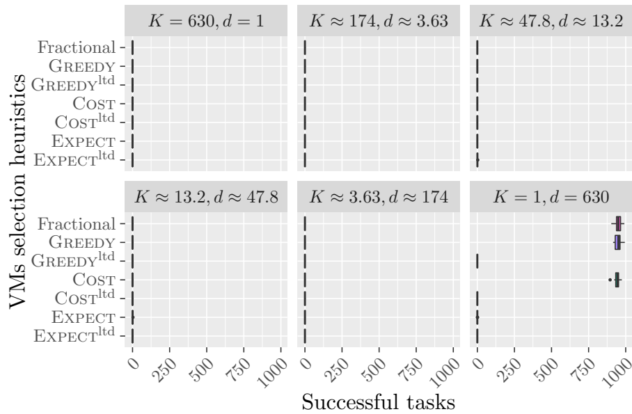
Figure 28: Number of successfully executed tasks of different methods to choose VMs when interrupting tasks with heuristic OPTRATIO. Platforms are generated with m_j = 10 , M = 60 , c_j = s_j , b = 630 . The values for d and K follows a geometric progression between 1 and b = 630 . Execution times follow a half-normal distribution.
