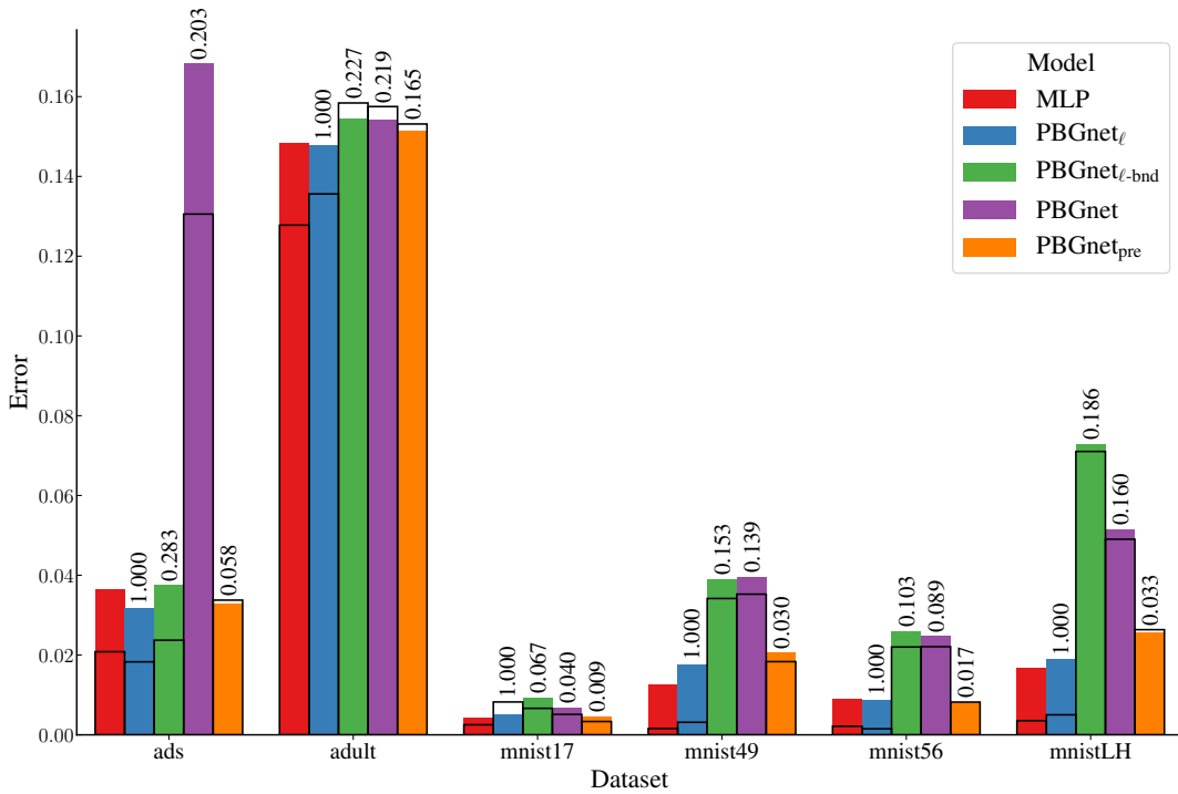
Figure 4: Visualization of experiment results for the models on the binary classification datasets. The colored bars display the test error while the black outlined bars exhibit the train error. The PAC-Bayesian generalization bounds are identified on the top of the bars and hold with probability 0.95.
