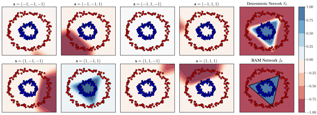
Figure 3: Illustration of the proposed method in Section 3 for a one hidden layer network of size d_1 = 3 , interpreted as a majority vote over 8 binary representations s \in \{-1, 1\}^3 . For each s , a plot shows the values of F_{w_2}(s)\Psi_s(\mathbf{x}, \mathbf{W}_1) . The sum of these values gives the deterministic network output F_\theta(\mathbf{x}) (see Equation 9). We also show the BAM network output f_\theta(\mathbf{x}) for the same parameters \theta (see Equation 6).
