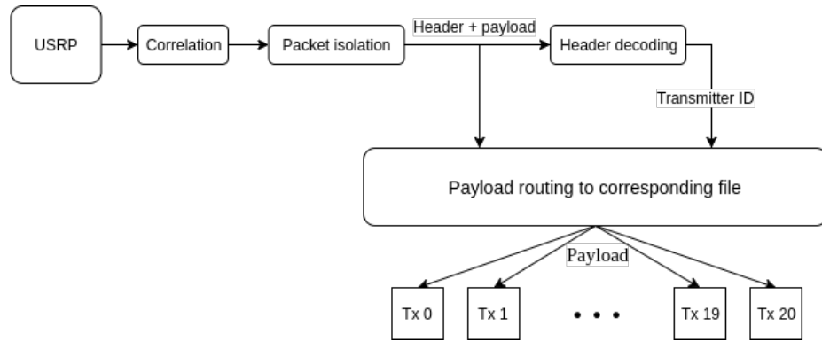
Fig. 3. Reception flowgraph
