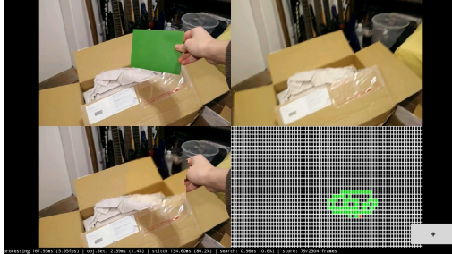
Fig. 9: Split view containing (from top left to bottom right): camera input, fill frame, (inpainted) output frame, frame store array
