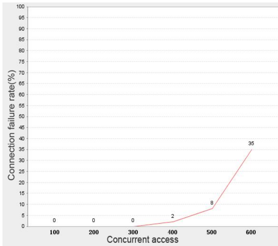
Figure.3. The connection failure rate varies with concurrent access numbers
